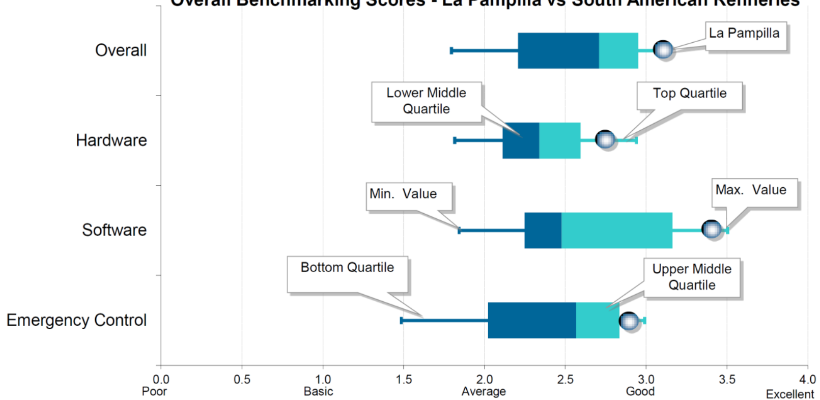
Overall Benchmarking Scores - La Pampilla vs South American Refineries
