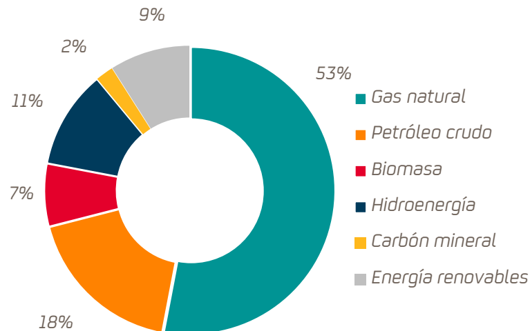
2040 = 54.0 Mtep
