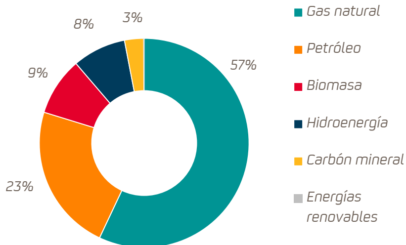
2013 = 29.2 Mtep
